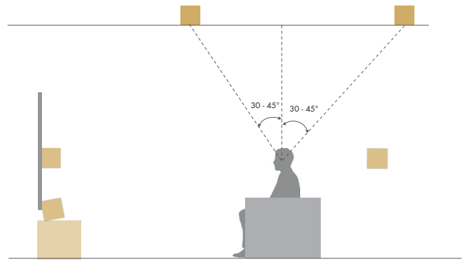
Reference listening position and speaker placement
