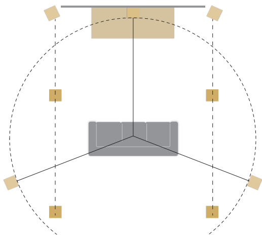
Reference listening position and speaker placement
